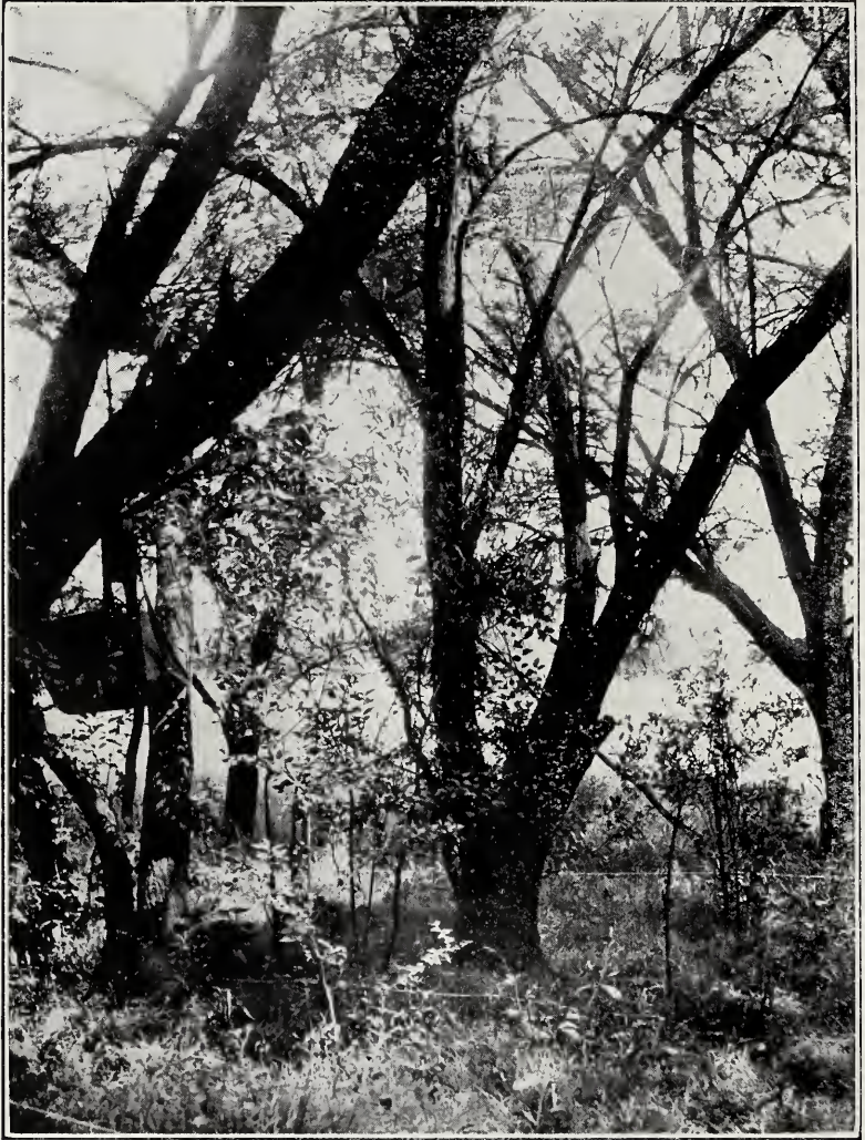
PLATE 11. Acacia bush. Inside view of portion of the belt transect, Fig. IX. Portions of three of the transverse lengths of cord of the transect can be seen. The large trees are Acacia Karroo . The taller sapling with narrow leaves, centre, is Rhus lancea ; another individual of it can be seen to the right. The others are Celtis rhannifolia . In the right foreground is an individual Achyranthes aspera . The ground vegetation is mainly composed of Bromus unioloides and Ehrharta crecta .
